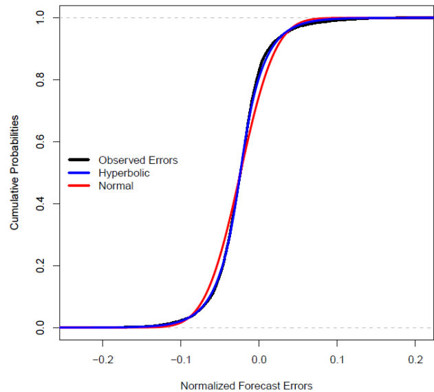
Fig. 5: A cumulative distribution plot of the NYISO day-ahead load forecast errors, along with the Gaussian and hyperbolic model distributions.
