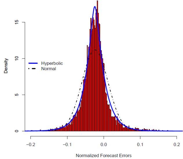
Fig. 4: A histogram of the distribution of day-ahead load forecasting errors for the NYISO system, normalized by the yearly average load. \mu = -0.024 ; \sigma = 0.036 ; \gamma = 0.379 ; \kappa = 3.799 . A Gaussian distribution with the same mean and standard deviation is shown along with a hyperbolic distribution fit to the observed data.
