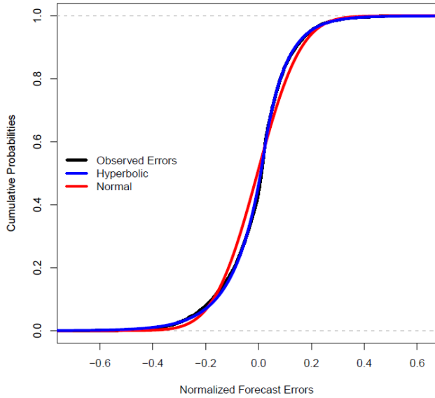
Fig. 10: A cumulative distribution plot of the CAISO day-ahead wind power forecast errors, along with the Gaussian and hyperbolic model distributions.
