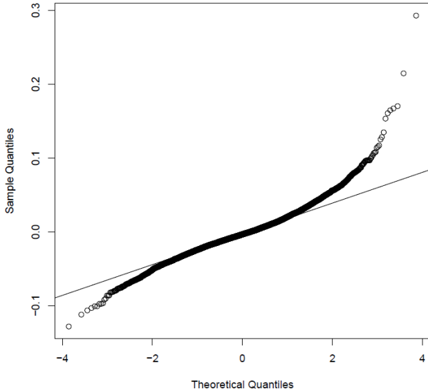
Fig. 3: A normal quantile-quantile plot of the distribution of day-ahead load forecasting errors for the CAISO system, normalized by the yearly average load. The line runs through the first and third quantiles of the observed distribution.
