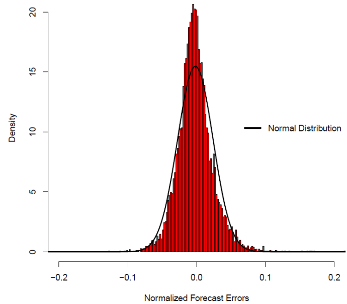
Fig. 2: A histogram of the distribution of day-ahead load forecasting errors for the CAISO system, normalized by the yearly average load. \mu = -0.002 ; \sigma = 0.026 ; \gamma = 0.715 ; \kappa = 4.725 .
