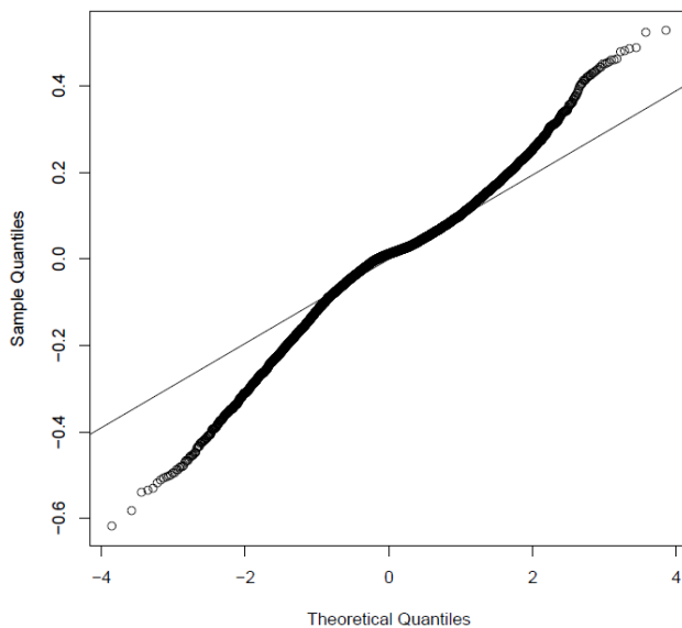
Fig. 8: A normal quantile-quantile plot of the distribution of day-ahead wind power forecasting errors for the CAISO system, normalized by the installed wind power capacity.
