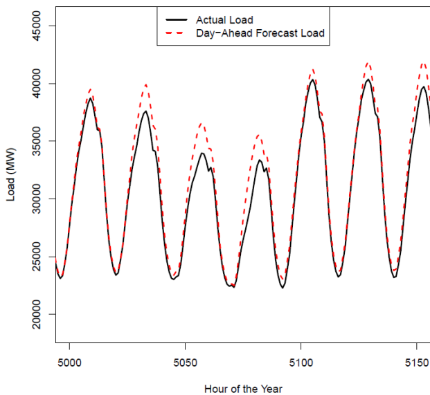
Fig. 1: Hourly load and forecast load values for one week in the CAISO system.
