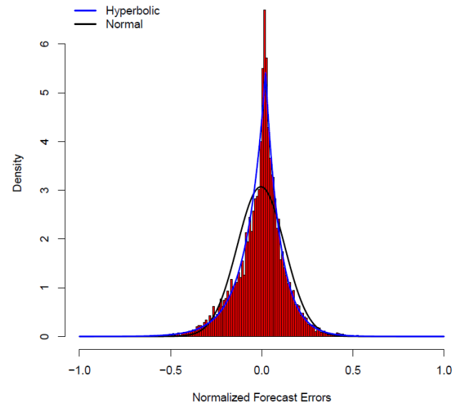
Fig. 9: A histogram of the distribution of day-ahead wind power forecasting errors for the CAISO system, normalized by the installed wind capacity. \mu = -0.004 ; \sigma = 0.130 ; \gamma = -0.393 ; \kappa = 1.503 . A Gaussian distribution with the same mean and standard deviation is shown along with a hyperbolic distribution fit to the observed data.
