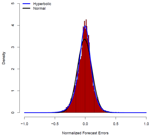
Fig. 11: A histogram of the distribution of day-ahead wind power forecasting errors for the ERCOT system, normalized by the installed wind capacity. \mu = -0.012 ; \sigma = 0.119 ; \gamma = -0.062 ; \kappa = 1.030 . A Gaussian distribution
