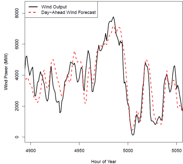
Fig. 6: Hourly wind power output and forecast wind power values for one week in the ERCOT system.
